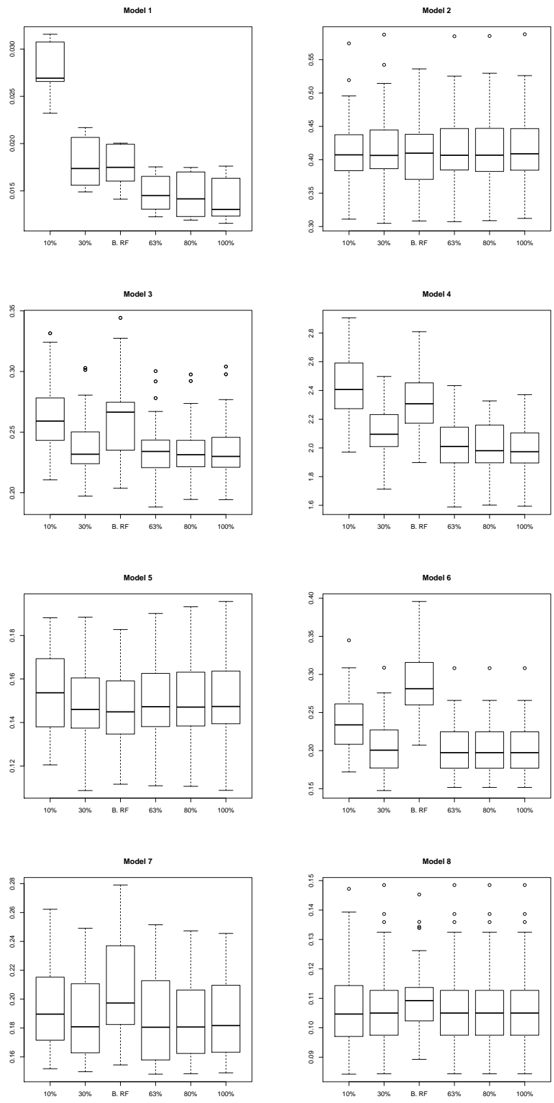
Figure 4: Comparison of standard Breiman's forests against several pruned Breiman forests in terms of L^2 error.
