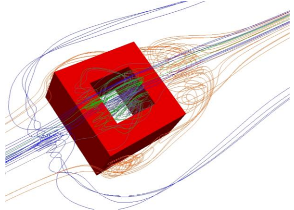
Figure 3: Flow structures within and around the patio
