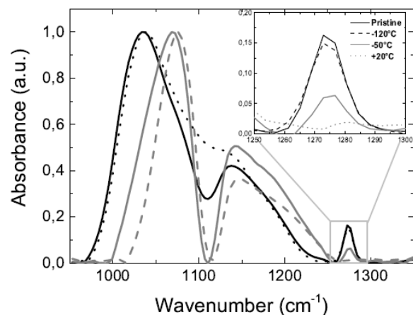
Fig. 1 FTIR analysis after a SF 6 plasma process with self-bias voltage for three different temperatures (-120°C, -50°C and +20°C) after a 15 min annealing at 350°C.
