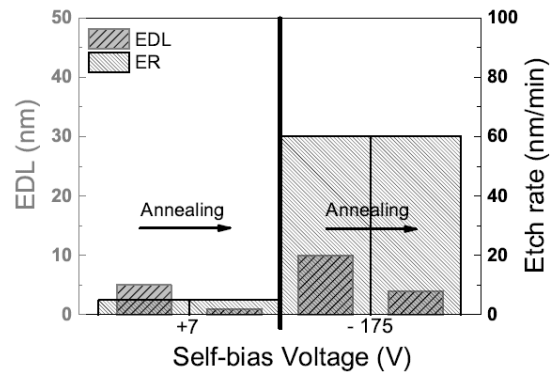
Fig. 3 OSG2.2 etch rate and EDL thickness plasma process (3Pa, 30sccm SF 6 , 10sccm C 4 F 8 ) with (-175V) or without self-bias voltage (+7V), -120°C before and after annealing.
