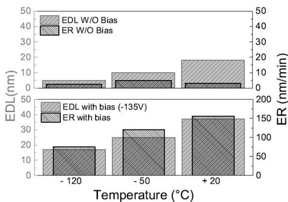
Fig. 2 OSG2.2 etch rate and EDL thickness for three different substrate temperatures after a plasma process (3Pa, 50sccm SF 6 ) with or without self-bias voltage
