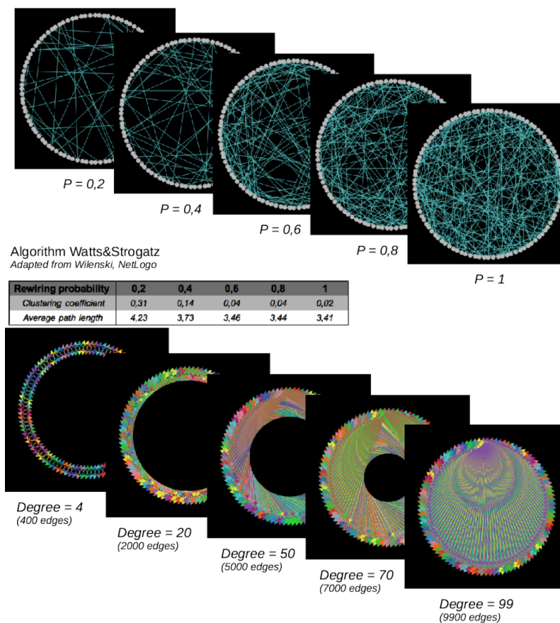
Figure 8. Small-world (top) and regular networks (below). Number of nodes = 100. Small-world networks are random networks (in the sense that edges are defined randomly, based on the “rewiring probability”) characterized by short average path lengths and high clustering coefficients, varying with the “rewiring probability”, while the number of edges is held constant. Regular networks are characterized by an increasing number of edges here.
