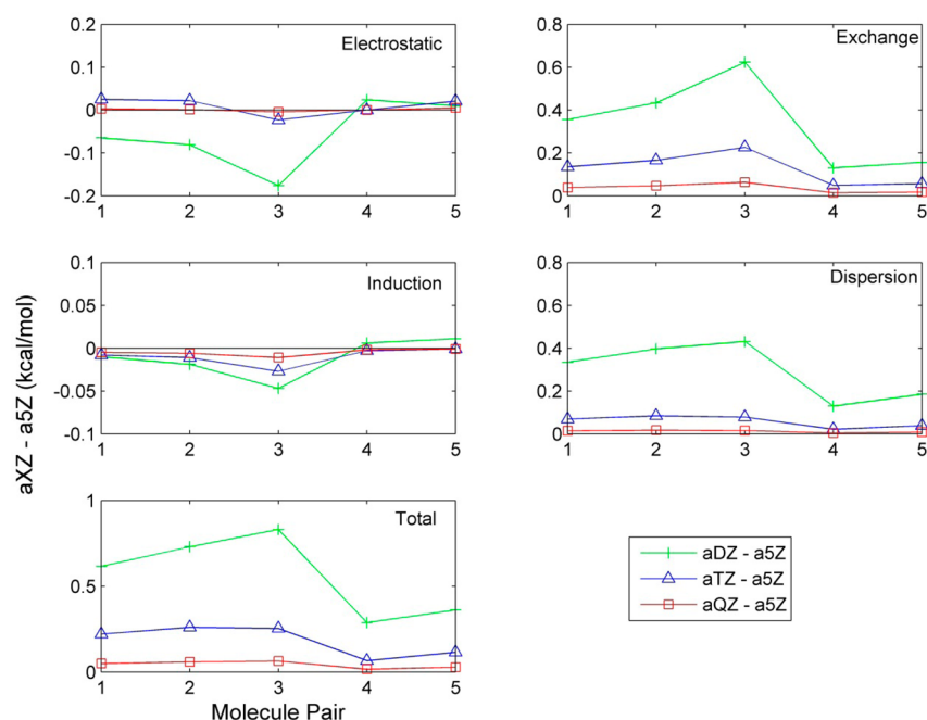
Figure 2. Difference between the SAPT2+ energy components calculated using aug-cc-pVXZ ( X = D, T, and Q ) basis set with the value obtained using aug-cc-pV5Z.
