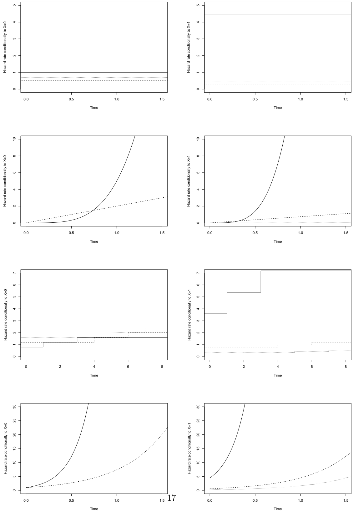
Figure 1: Conditional hazard rates in simulated data for Scenarios 1 to 4 from top to bottom. Solid line: hazard in segment 1. Dash line: hazard rate in segment 2. Dot line: hazard rate in segment 3.
