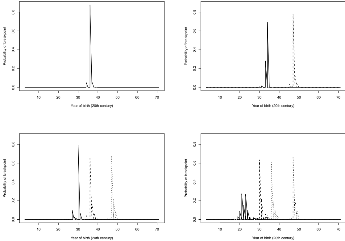
Figure 2: Marginal distributions of the breakpoints in the models with one, two, three and four breakpoints. The maximum a posteriori for the breakpoints are respectively: top left 1936, top right 1934 and 1947, bottom left 1930, 1936 and 1947, bottom right 1921, 1930, 1936 and 1947.
