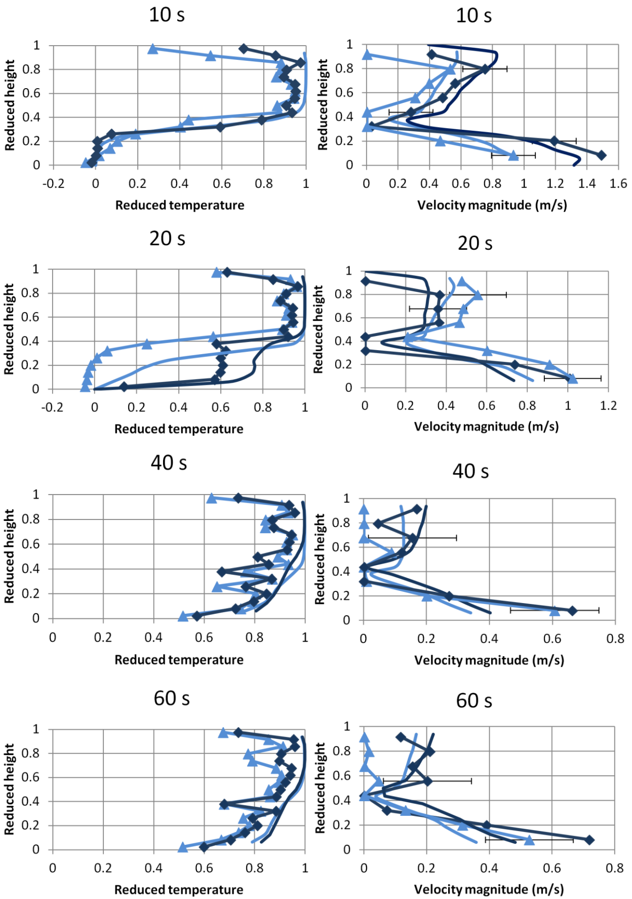
Figure 14: Influence of initial temperature on temperature and velocity profiles in the symmetry plane. Experiences: ▲ T_i=273 K ◆ T_i=253 K, Model: — T_i=273 K — T_i=253 K.
