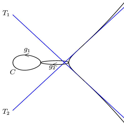
FIGURE 1. Real picture of the curve \mathcal{T} .
