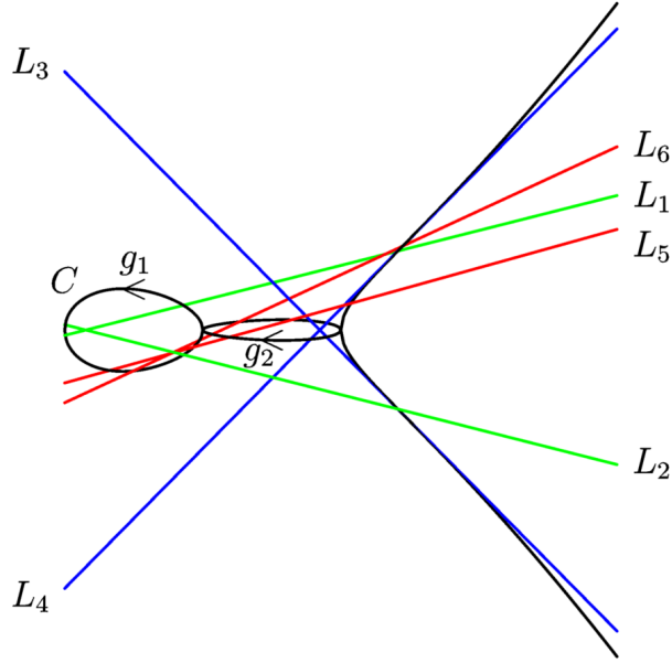
FIGURE 3. Representation of the curve C_7 over the segment x = (-1; 3) .
