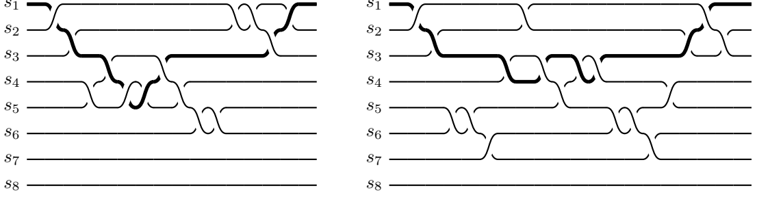
FIGURE 5. The braids \Sigma_1 and \Sigma_2 . The thick strands correspond to the cycles g_1 and g_2 , respectively.
