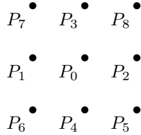
FIGURE 4. Representation of the nine inflexion points of C in (\mathbb{F}_3)^2 .
