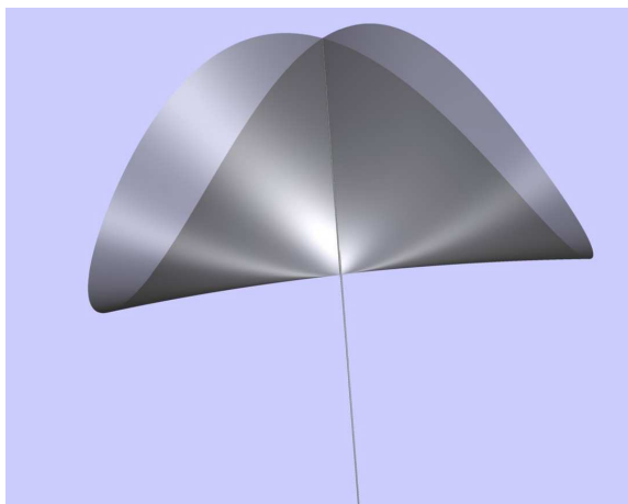
FIGURE 2. Whitney umbrella.
