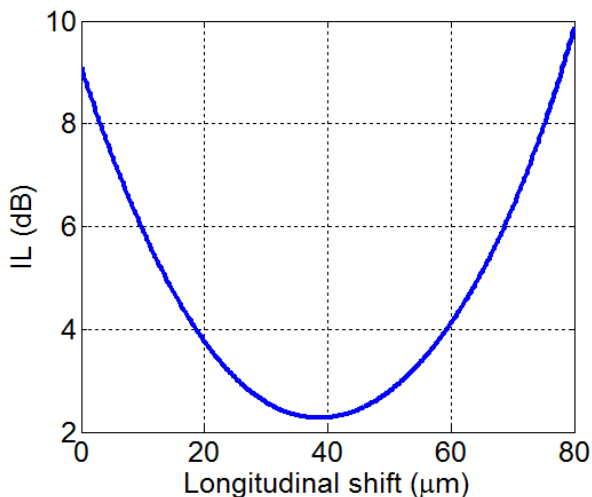
Figure 7: Insertion loss as a function of the longitudinal shift of the two tapers for \lambda = 1550 nm. The gap between the two waveguide layers is 1000 nm. The optimized longitudinal shift is of about 40 \mu\text{m} ; the corresponding insertion loss is 2.3 dB.
