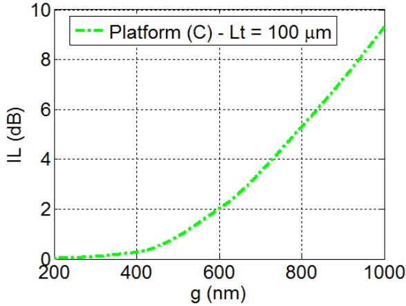
Figure 6: Insertion loss of a vertical tapered link fabricated on the platform (C) with taper length L_t = 100 \mu\text{m} and for \lambda = 1550 nm. The distance g between the layers is progressively increased from 200 nm to 1000 nm. As the distance increases, the insertion loss grows with an almost quadratic trend.
