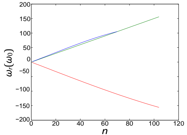
Fig. 2. Real frequency of the trapped electron (resp. ion) modes in red (resp. in blue) plotted against the toroidal mode number n . The green line is \omega = \frac{3}{2} \eta and corresponds to the marginal TIM mode [9].
