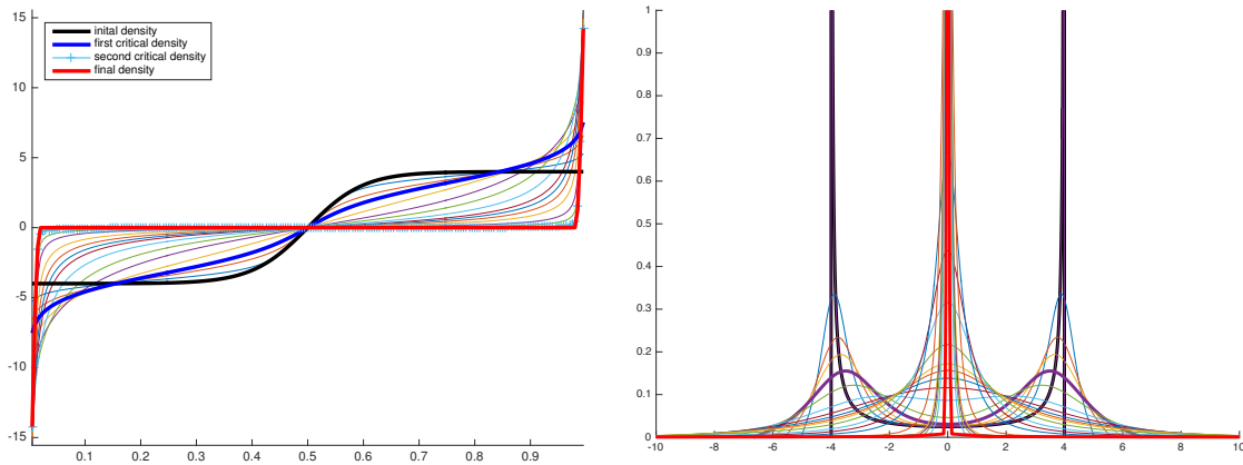
FIGURE 3. Density and repartition functions.
