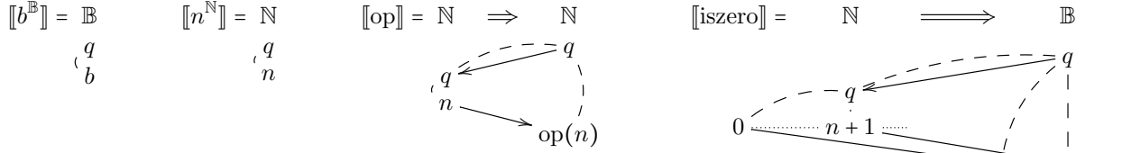
Fig. 3. Interpretation of the basic combinators of PCF
