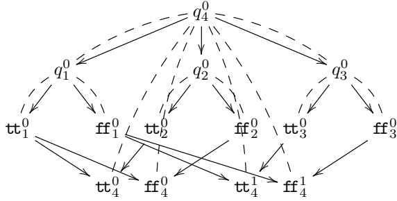
Fig. 2. The reduced pre-strategy for \text{if} : \mathbb{B}_1 \Rightarrow \mathbb{B}_2 \Rightarrow \mathbb{B}_3 \Rightarrow \mathbb{B}_4
