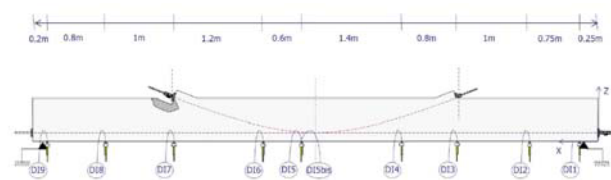
Figure 2: Location of the second network of displacement transducers
