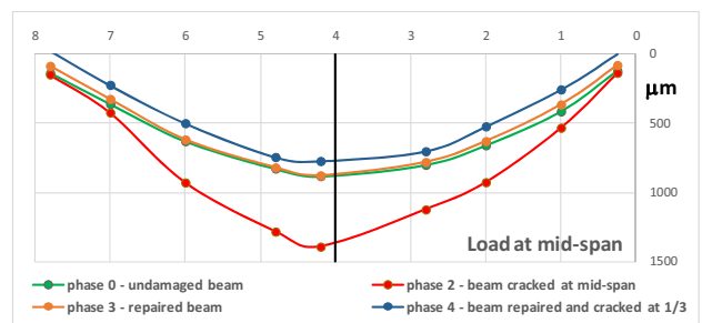
Figure 7: Deflections under three-point bending at mid-span
