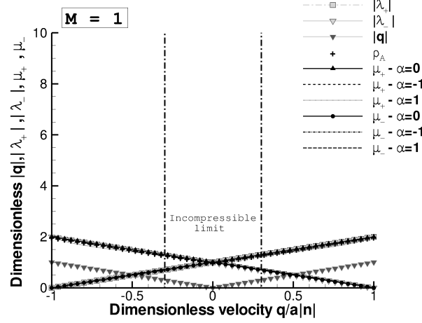
Figure 3: Dimensionless eigenvalues for the original matrix-valued dissipation (Roe) and for the rescaled Roe scheme when M = 1
