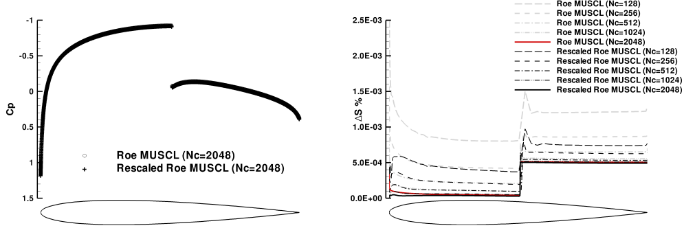
Figure 10: Comparison of the flow solution for the Roe scheme and the rescaled Roe scheme at M_\infty = 0.8 , \alpha = 0^\circ . Left: pressure coefficient. Right: entropy distribution
