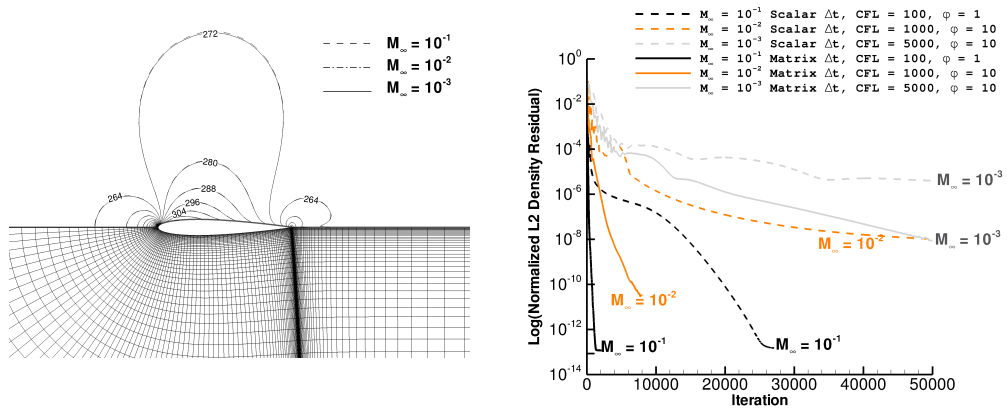
Figure 9: Effect of grid stretching on the rescaled Roe scheme. Left: Velocity contours with the inflow Mach number. Right: Convergence history for the scalar (dashed lines) and the matrix (solid lines) time steps
