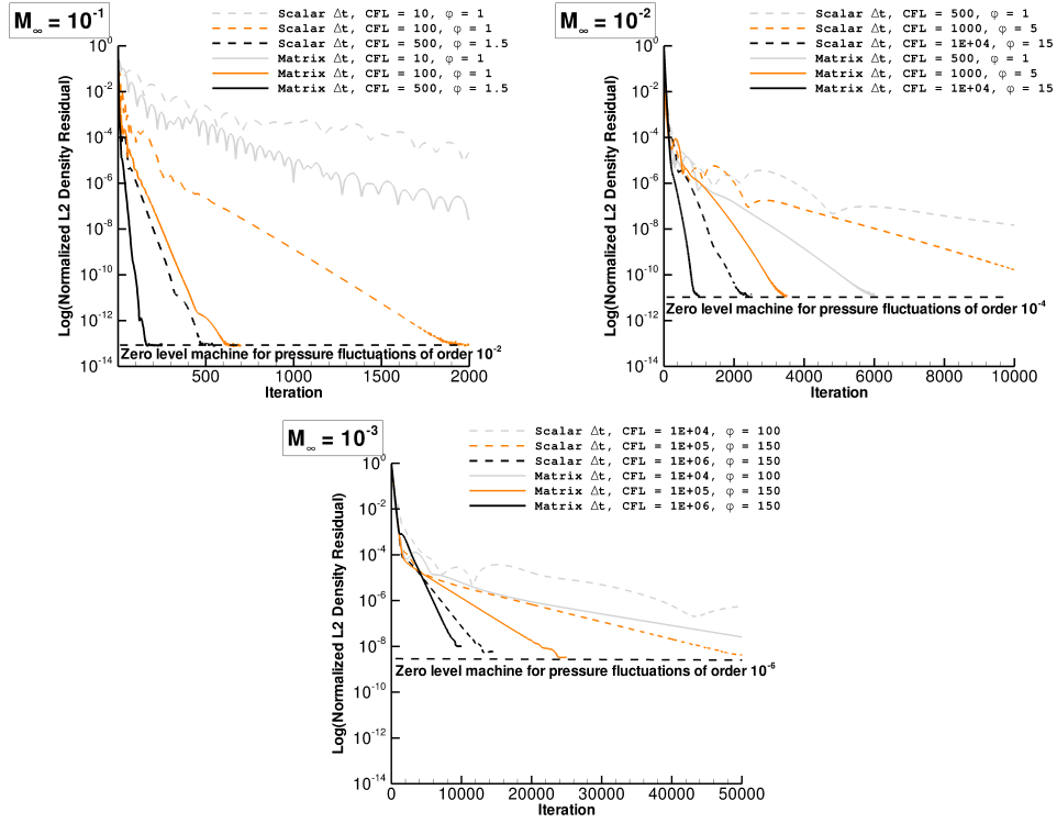
Figure 8: Convergence history for the rescaled Roe scheme with the inflow Mach number 10^{-1} , 10^{-2} and 10^{-3} . Solid lines: matrix time-step. Dashed lines: scalar time step
