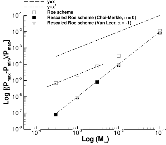
Figure 7: Pressure fluctuations with the inflow Mach number for the Roe scheme and the rescaled Roe scheme
