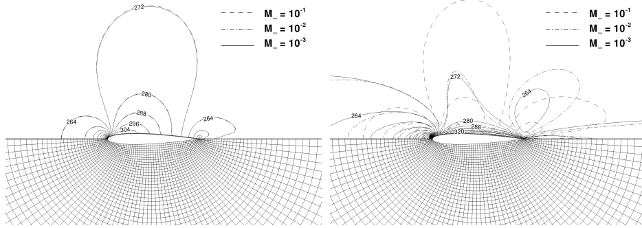
Figure 5: Velocity contours with the inflow Mach number in the Vasseberg-Jameson mesh. Left: rescaled Roe scheme. Right: Roe scheme ( V_\infty = 270 \text{ m/s} )
