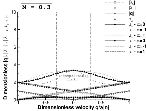
Figure 2: Dimensionless eigenvalues for the original matrix-valued dissipation (Roe) and for the rescaled Roe scheme when M = 0.3
