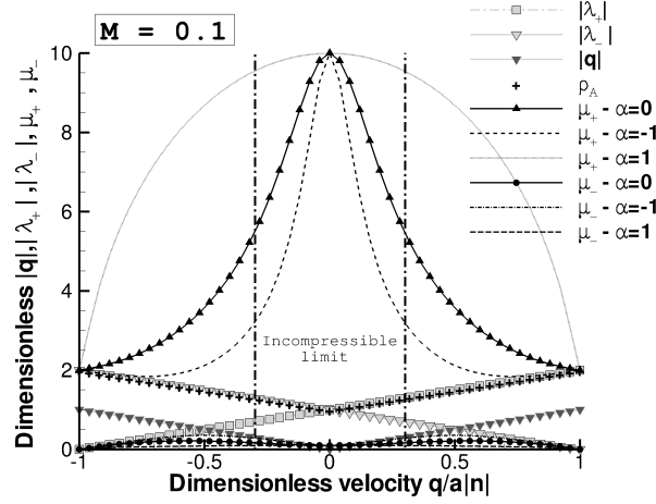
Figure 1: Dimensionless eigenvalues for the original matrix-valued dissipation (Roe) and for the rescaled Roe scheme when M = 0.1
