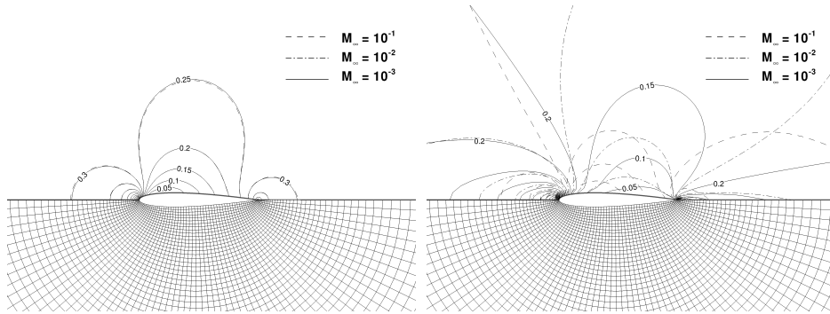
Figure 6: Contours of the normalized pressure with the inflow Mach number in the Vasseberg-Jameson mesh. Left: rescaled Roe scheme. Right: Roe scheme
