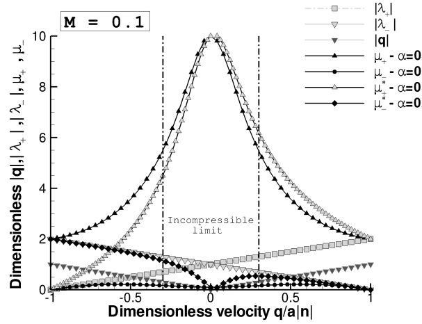
Figure 4: Dimensionless corrected eigenvalues \mu_{\pm}^* in the definition of time-step matrix when M = 0.1 - Grey delta symbols: \mu_+^* . Black diamond symbols: \mu_-^*
