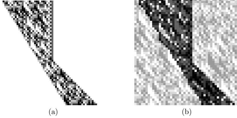
Figure 4: . (a) Space-time diagram of F_{3,2} starting from a configuration with a finite number of non-zero cells (time goes from bottom to top, states are represented by tones of grey from white for 0 to black for 5). (b) Space-time diagrams of F_{3,2} starting from two random asymptotic configurations (the coincident cells are colored with light grey tones, the effect of the perturbation is colored with dark grey tones)
