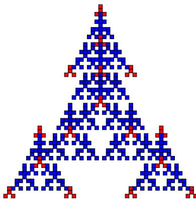
Figure 6: Simulation of \oplus_2 with a triangular neighborhood at iteration 25 starting from an initial configuration with a single 1 inside 0s: cells in state 1 are in red, cells that have been in state 1 between iteration 0 and 24 but not at 25 are in blue, and the others cells are not drawn.
