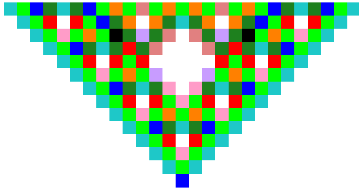
Figure 2: In the first row some space-time diagrams of \Psi are shown (state (0, 0) is represented by empty space). The third diagram shows the morphisms representing the dependence of \Psi^t(c^{(a,b)})_i on (a, b) , for each space-time coordinate (i, t) : in particular, white means no dependence and red means bijective dependence.
