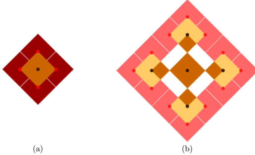
Figure 5: (a) Represents the evolution from iteration 0 to 2^k . Non-null cells at iterations 0 and 2^{k-1} are marked with dark brown and red dots, respectively (cell (0,0) is active at both instants). The balls of radius 2^{k-1} around these cells are colored with similar lighter colors. (b) Represents the evolution from iteration 2^k to 2^{k+1} . Dark brown dots represent non-null cells at iterations 2^k and 2^k + 2^{k-1} , while red dots represent the cells which are non-null at iteration 2^k + 2^{k-1} . The balls of radius 2^{k-1} around these cells are colored with similar lighter colors. Faded colors represent the cells outside the ball of radius 2^k .
