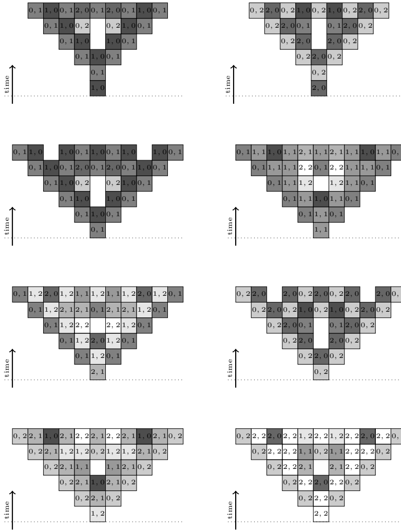
Figure 2: Some space-time diagrams of \Psi (state (0,0) is represented by empty space)
