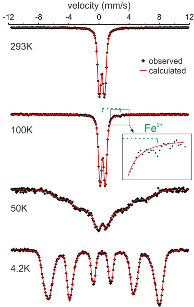
Figure 7: ^{57}Fe Mössbauer spectra of S3B sample recorded from room temperature down to 4.2 K.
