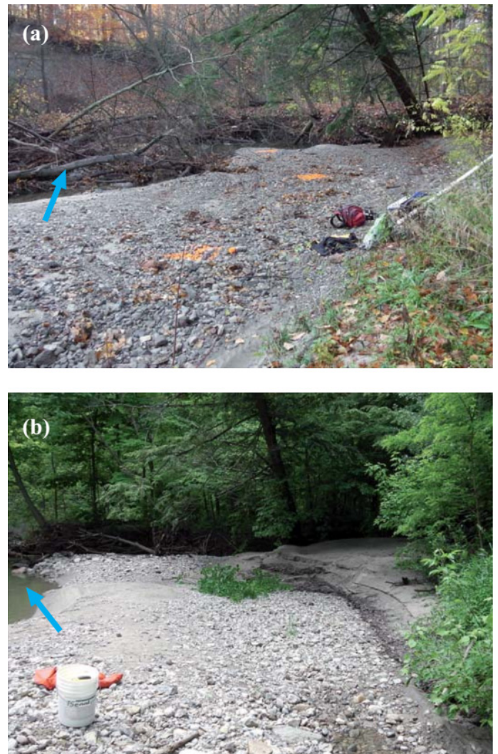
Figure 6. Strong modification of the bed on the upstream unrestored site (Control site, RK 0.35) before (a) and after (b) the May 29 th flood. (a) Picture taken on the 2012/10/26. (b) Picture taken on the 2013/06/13. Blue arrow indicates flow direction.
