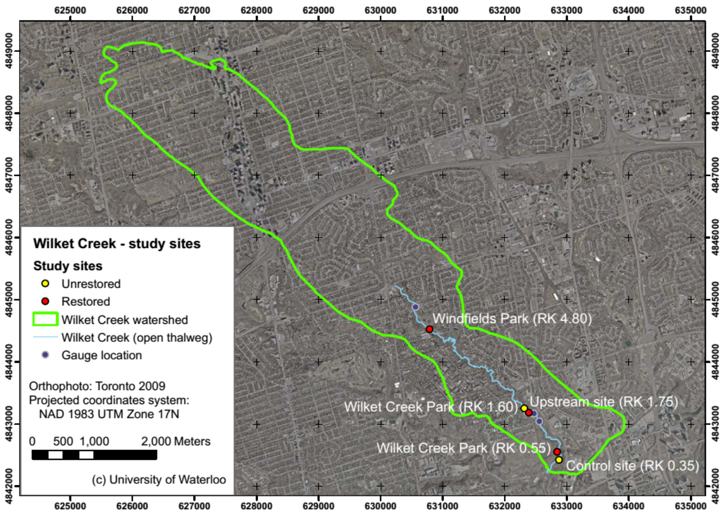
Figure 1. Location of the five study sites within the Wilket Creek catchment and indication of their river kilometer (RK). Wilket Creek is located within the suburban area of Toronto.
