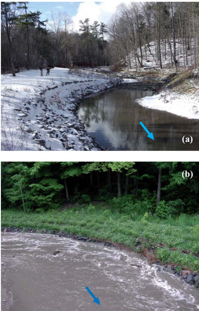
Figure 2. (a) Example of the restoration works in the main study site (Edwards Gardens, RK 1.60). The designed channel corresponds to a sinuous planform channel with riffle-pool features. Both embankments and riffles are made from exogenous material which size is greater than natural bed material. (b) Solicitation of the outer river bank by logs during a flashy flood (2013/06/13, Edwards Gardens, RK 1.60). Blue arrow indicates flow direction.
