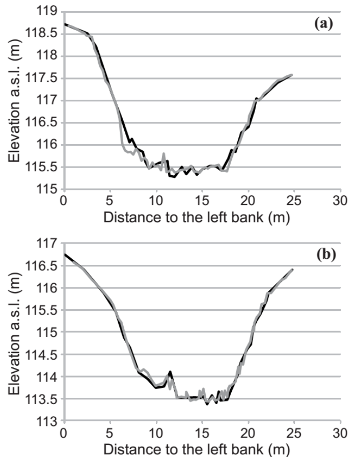
Figure 3. Topographic evolution of cross-sections 8 (subplot a) and 14 (subplot b) of the Wilket Creek Park site (RK 1.60) before (2013/02/01, black line) and after (2013/07/25, grey line) May 29 th flood. These results show overall stability of the designed channel with some lateral adjustments on cross-section 8.
