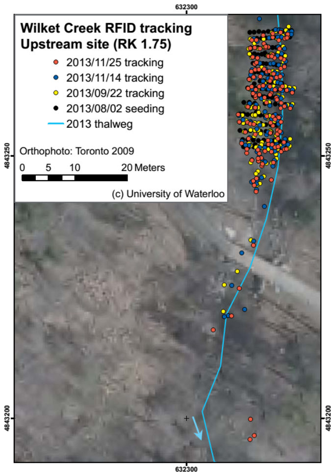
Figure 7. RFID tracking on the Upstream site (RK 1.75). The seeding locations of tracers are indicated. Tracers were naturally reworked between the seeding and the first tracking (2013/09/22) because of four flood events (maximum estimated discharge: 1.7 \text{ m}^3/\text{s} on 2013/08/26). Blue arrow indicates flow direction.
