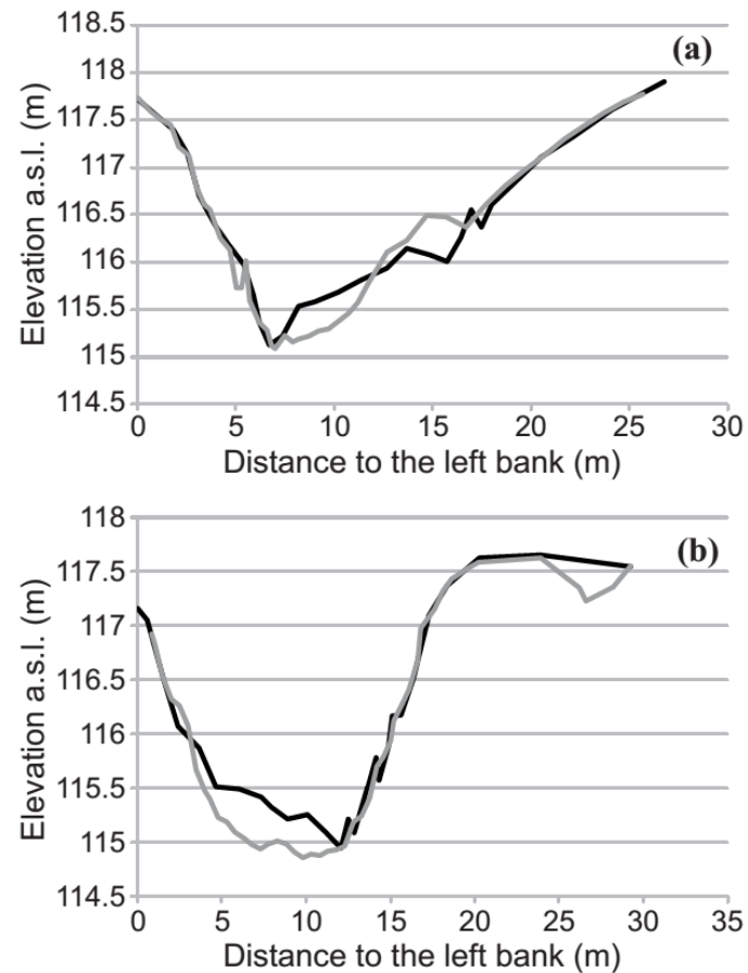
Figure 5. (a) Internal reworking of sediment (cross-section 6) between 2013/02/01 (black line) and 2013/07/25 (grey line) illustrating the effects of two over bankfull floods. (b) Flushing of fine sediments in pools (cross-section 9) between the same survey dates.
