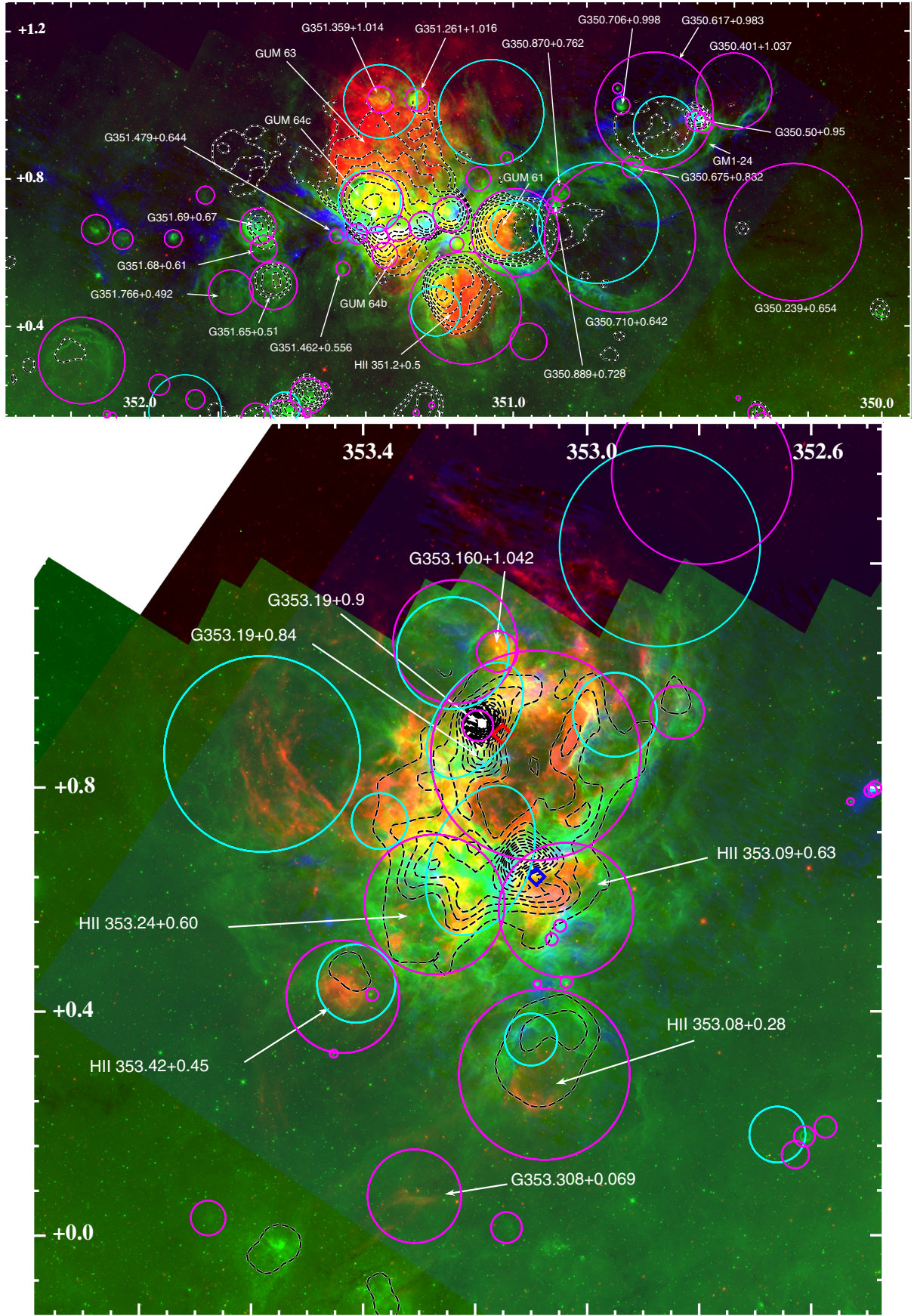
Fig. 1. H\alpha (red), GLIMPSE-8 \mu\text{m} (green), and SIMBA-1.2 mm (blue) composite image of NGC 6334 ( upper panel ) and NGC 6357 ( lower panel ). The quoted coordinates are galactic coordinates. The overlaid isocontours are from SGPS radio emission. The purple and cyan circles show the H II regions from Anderson et al. (2014) and Langston et al. (2000) respectively. For NGC 6357, the position of stellar clusters Pismis 24 (red diamond) and AH03J1725-34.4 (blue diamond) are also indicated.
