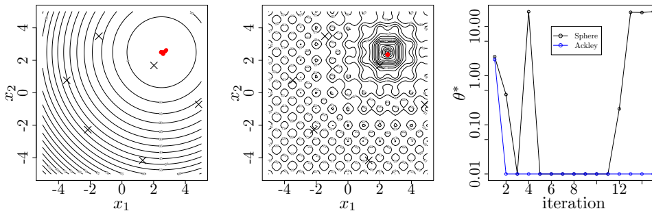
Figure 7: DoEs created by the toy greedy algorithm 2 after 15 iterations on the Sphere (left) and the Ackley (middle) functions. Right: plot of “best” length-scale, \theta^* . The initial DoE is different from the one shown in Figure 5.
