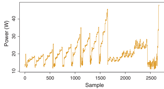
Fig. 6. Synthetic workload's power profile.
