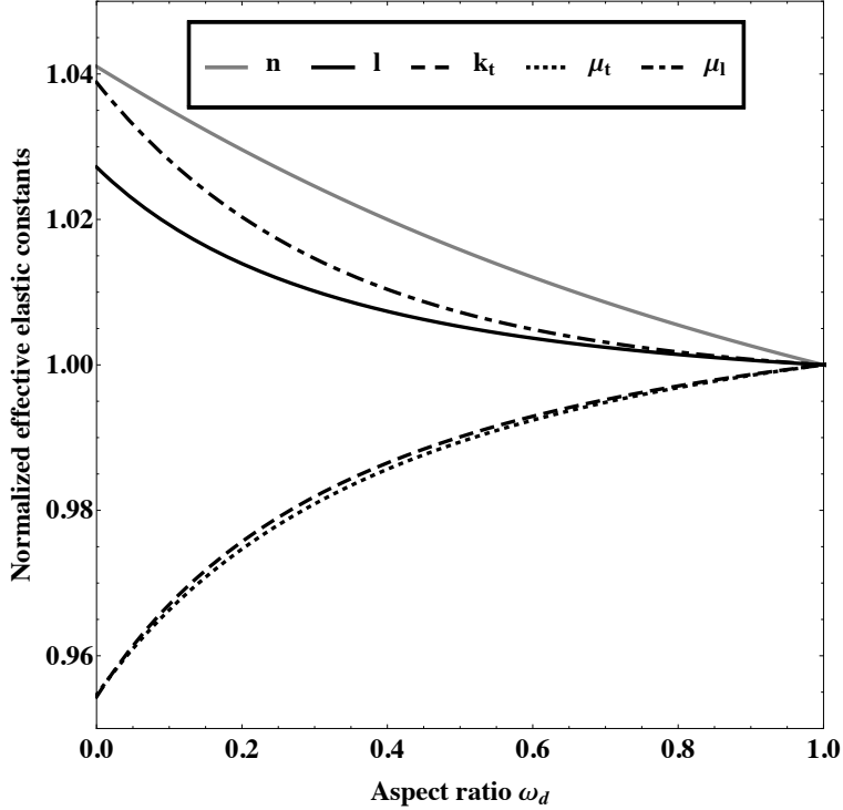
Figure 4: Effective elastic constants as a function of the aspect ratio for an oblate spheroidal spatial distribution of the centers of the pattern \mathcal{S} . The total porosity f is equal to 25 % and the radius of the voids is 1 nm.
