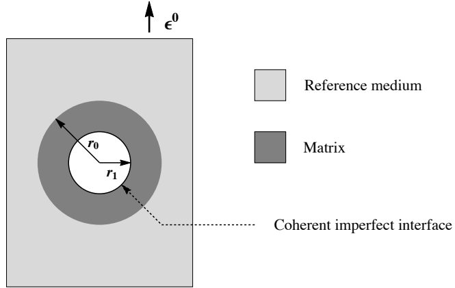
Figure 2: Problem of the heterogeneous inclusion in an infinite reference medium for spherical nano-voids with the interface stress model.
