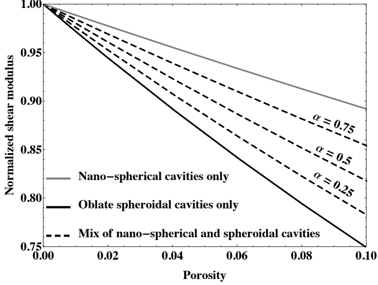
Figure 9: Normalized effective shear modulus as a function of the total porosity. Aspect ratio of the microvoids \omega = 0.2 . Radius of the spherical nanovoids r = 1 nm.
