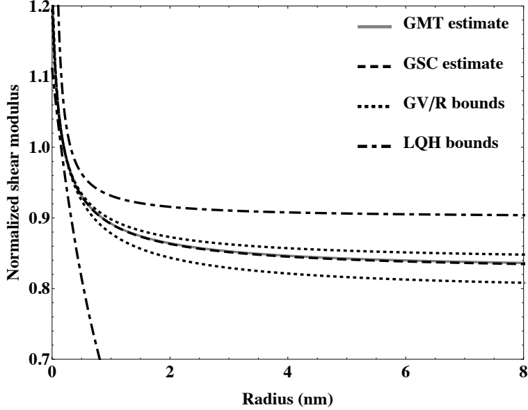
Figure 3: Effective shear modulus (normalized with respect to the shear modulus of the matrix) as a function of the radius of the cavities. The total porosity f is equal to 5 %. The models are evaluated by setting f_S = f .
