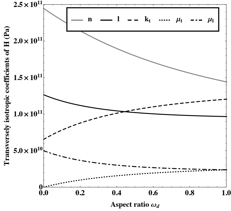
Figure 6: Transversely isotropic constants of \mathbb{H} as a function of the aspect ratio for an oblate spheroidal spatial distribution of the centers of the pattern \mathcal{S} . The total porosity f is equal to 25 % and the radius of the voids is 1 nm.
