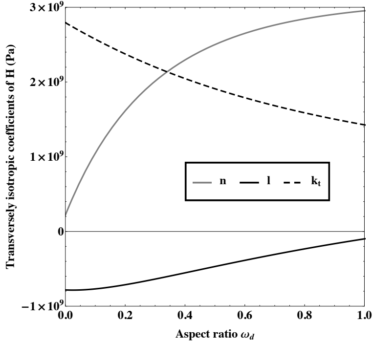
Figure 7: Transversely isotropic constants of \mathbb{H} as a function of the aspect ratio for an oblate spheroidal spatial distribution of the centers of the pattern \mathcal{S} . The total porosity f is equal to 25 % and the radius of the voids is 1 nm. Specific case where E_m = 100 GPa, \nu_m = 0.2 , k_s = 50 N/m, \mu_s = 30 N/m.
