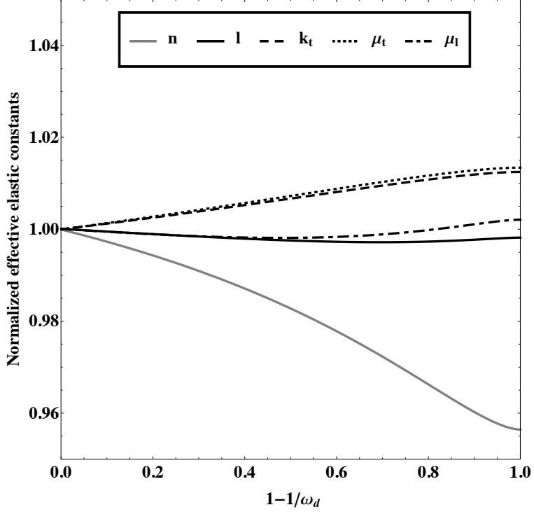
Figure 5: Effective elastic constants as a function of the aspect ratio for a prolate spheroidal spatial distribution of the centers of the pattern \mathcal{S} . The total porosity f is equal to 25 % and the radius of the voids is 1 nm.
