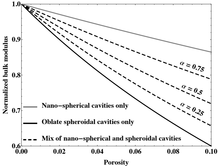
Figure 8: Normalized effective bulk modulus as a function of the total porosity. Aspect ratio of the microvoids \omega = 0.2 . Radius of the spherical nanovoids r = 1 nm.
