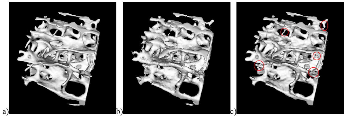
Figure 1 : Illustration of joint segmentation/super resolution applied to a 3D bone micro image : a) original image, voxel size 20µm, b) low resolution image including undersampling by a factor 2 and additive Gaussian noise ( \sigma=0.1 ), c) restored 3D binary image. The red circles show that the method has allowed the restoration of the connectivity that was lost after undersampling
