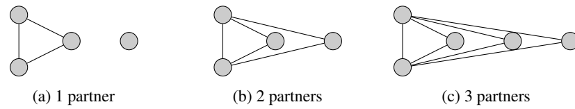
Figure 15: Shared partners
