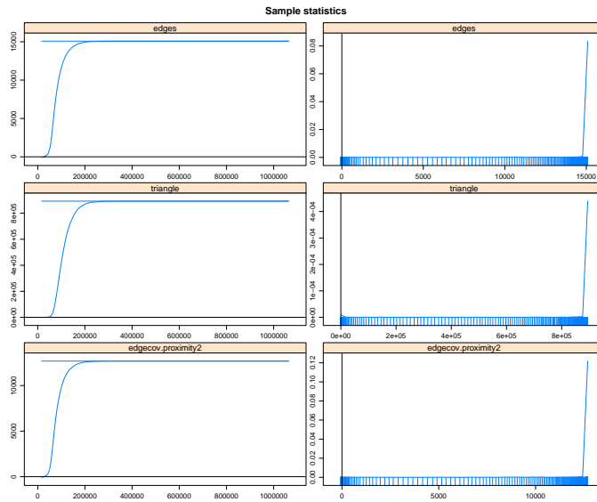
Figure 11: Goodness of Fit diagnostics, bad example
