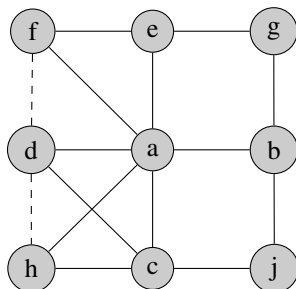
Figure 3: Node level dependence illustration: the Markovian neighborhood
