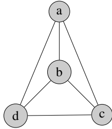
Figure 4: Markov graph
