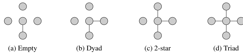
Figure 14: K-stars
