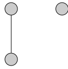
Figure 14: Dyad
