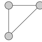
Figure 16: Triad
