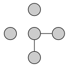
Figure 19: 2-star
