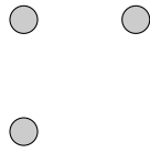
Figure 13: Empty
