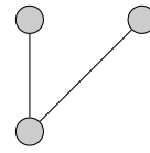
Figure 15: 2-star
