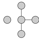
Figure 20: 3-star
