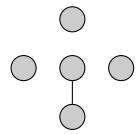
Figure 18: 1-star
