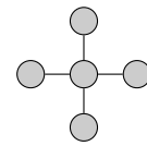
Figure 21: 4-star
