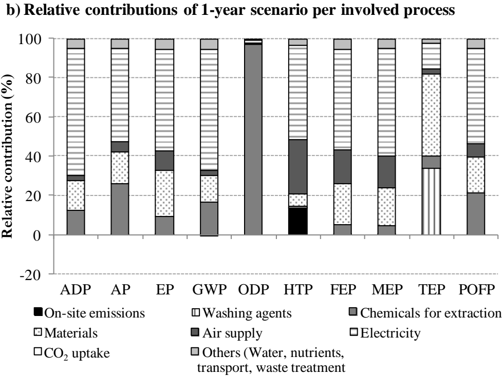
Figure 2. Relative contributions of the semi-continuous production of essential terpene oils by O. secundiramea to each impact category per a) stage and b) process involved.
