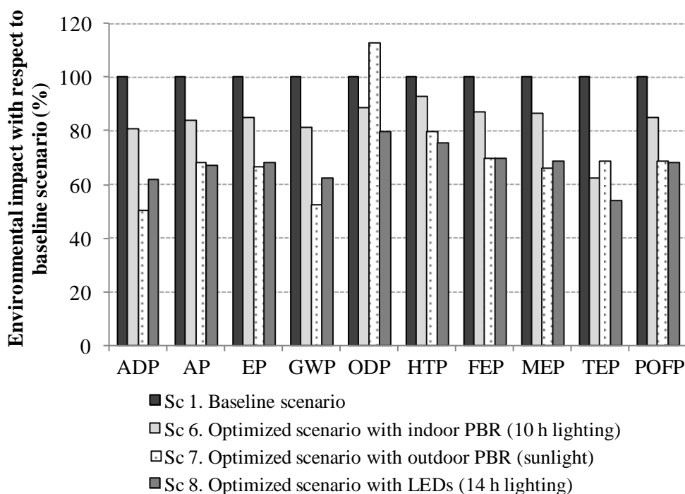
Figure 7. Environmental profile of the optimized scenarios (including energy reduction and improved downstream processing) for the production of essential terpene oils by O.
