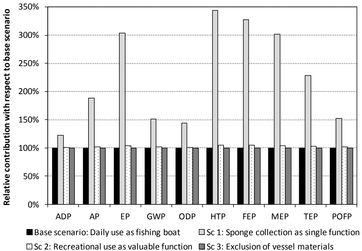
15 16 Figure 7 Effect of vessel operations in the environmental profile of the production of pure crambescin 17 and crambescidin.
