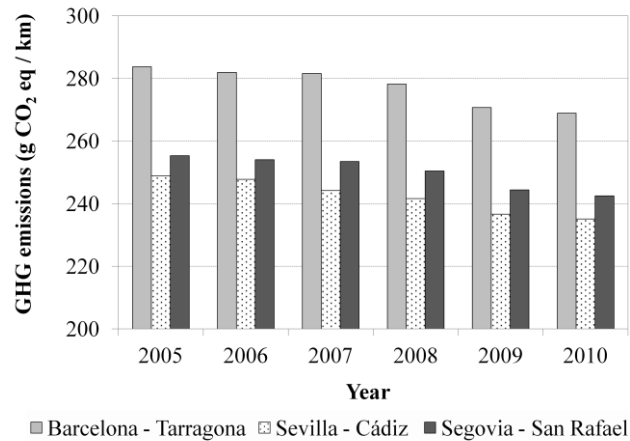
Figure 2. Average GHG emissions per km travelled in each motorway stretch for average speeds of 120 km/h and 85 km/h for light and heavy vehicles
