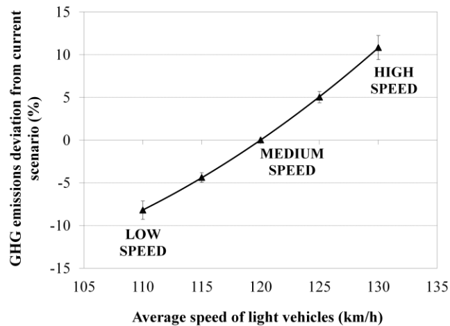
Figure 6. Average effect of speed of light vehicles on total GHG emissions
