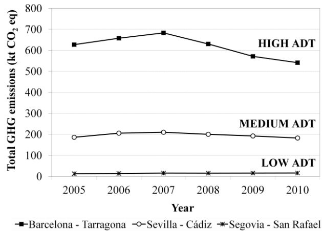
Figure 1. Evolution of total GHG emissions for three motorway stretches during 2005-2010 for average speeds of 120 km/h and 85 km/h for light and heavy vehicles
