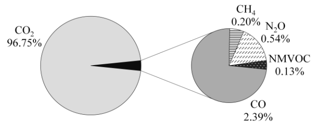
Figure 4. Average contribution of each gas to the total 100-year GWP
