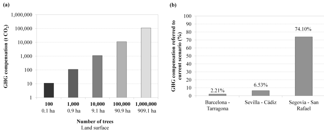
Figure 5. GHG compensation potential of forest species: tons of CO 2 vs number of trees and land surface (a) and CO 2 reduction percentage of 100,000 trees with respect to total GHG emissions per year (b)
