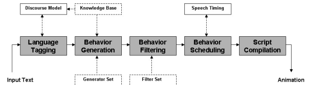
Fig. 3: Architecture of BEAT toolkit [18]
