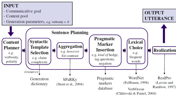
Fig. 2: Architecture of PERSONAGE generator [60]
