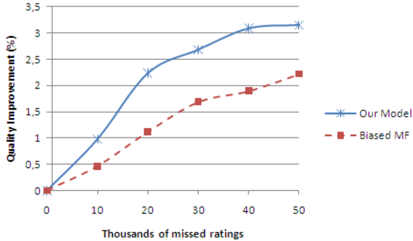
Figure 4: Quality's improvement by new ratings
