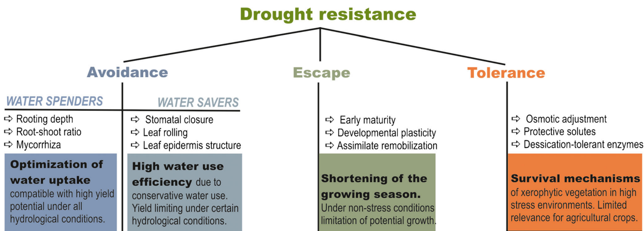
Fig. 6 Drought resistance according to Levitt (1980). Different resistance strategies, examples for corresponding adaptive traits and their potential use/limitation for agricultural crops. Drought avoidance via efficient water uptake is most compatible with high crop yields
