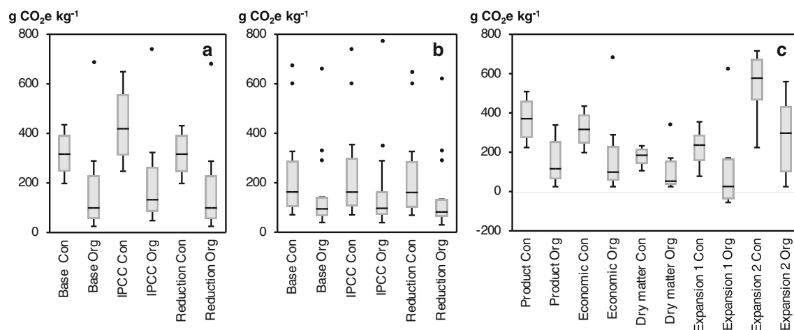
Fig. 3 Sensitivity analysis of the global warming potential ( \text{g CO}_2\text{e kg}^{-1} ) of conventional (Con) and organic (Org) management as affected by different estimations of nitrous oxide emissions in cereals ( a ) and open-air vegetables ( b ) and as affected by changes in coproduct consideration in cereals ( c ). Nitrous oxide scenarios are compared to Base , which represents base case sequestration using Mediterranean factors and include estimates using IPCC Tier 1 methodology (IPCC) and a 20 % reduction in the emission factor of organic fertilizers (Reduction). Coproduct scenarios include product allocation (Product), in which all
