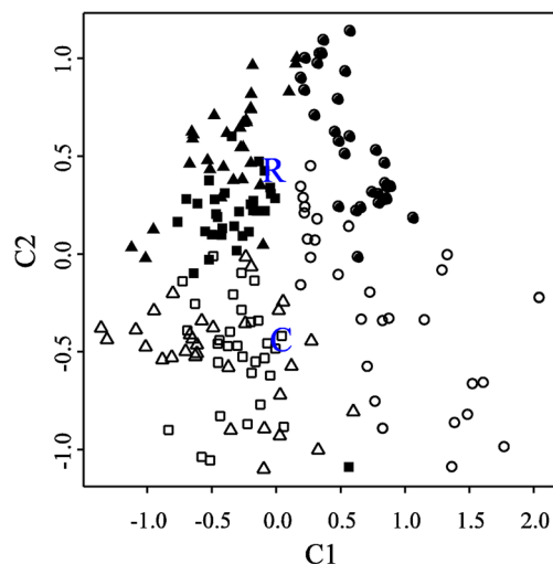
Fig. 3 Non-metric multidimensional scaling (NMDS) ordination plot. Each point represents a single weed community sample. The NMDS fits as much as possible the floristic dissimilarity between weed community samples in a two-dimensional plot to ease its visualization. Plotting symbols enable the visualization of the tillage system, i.e., reduced and conventional tillage, and the type of crop, i.e., wheat, spelt, and sunflower. The greater the dissimilarity between two weed communities, the more distant the respective symbols are in the plot. Filled symbols represent reduced tillage plots, and empty symbols represent conventional tillage plots. The labels R and C represent the centroids of reduced and conventional tillage, respectively. Circles , squares , and triangles represent sunflower, wheat, and spelt crops, respectively. The results show that weed communities surveyed under reduced tillage differ from those surveyed under conventional tillage. Moreover, weed communities found in the wheat and spelt crops are similar and both differ from those surveyed in the sunflower crop
