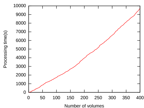
Figure 7: Processing time vs number of volumes
