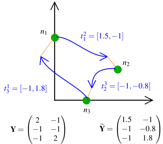
Figure 4: A simple problem with 3 volumes (green dots) and 3 translations: Blue arrows depict observed registrations, orange dotted lines represent registration error. Matrix \mathbf{Y} depicts ground truth transforms between all images. Matrix \tilde{\mathbf{Y}} represents estimated transforms.
