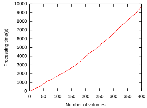
Figure 7: Processing time vs number of volumes
