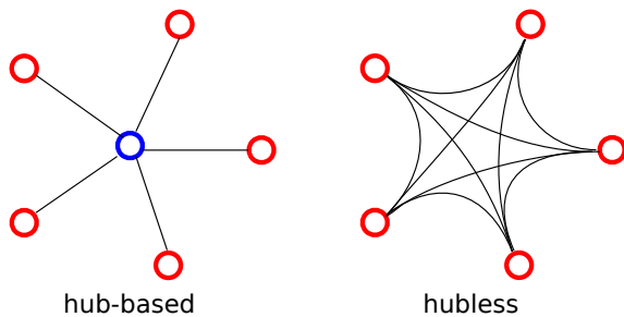
Figure 2: Fundamental differences between hub-based and hubless approaches. Here, 5 images are represented by 5 red dots. (Left) Hub-based approach : one needs a sixth image as a central model. This approach allows only 5 links between images, and its efficiency depends on the choice of the model image. (Right) The hubless approach : no image is picked as a model. This allows to compute 10 links between the 5 images.
