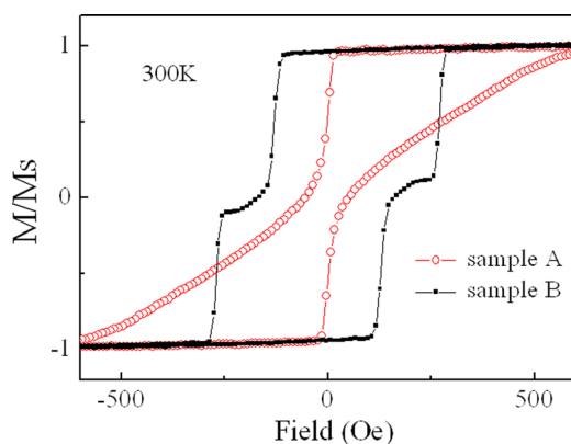
FIG. 1. Room temperature normalized magnetization vs field measurements of \text{Co(0.6)/[Ni(0.6/Co(0.3)]*3/AlOx(2.5)/[Co(0.2)/Ni(0.6)*3/Pt(y)/[Co(0.6)/Pt(1)]*3} MTJ under out-of-plane applied magnetic field with y = 1 (red open circle, sample A) and 2 nm (black solid square, sample B).
