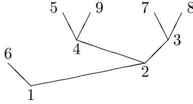
Fig. 1.2. Labeled strictly ordered binary tree.
