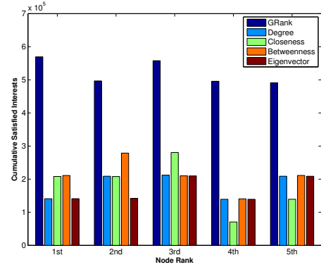
Figure 3: Cumulative Satisfied Interests by top identified nodes using each scheme over an average of five different simulations
