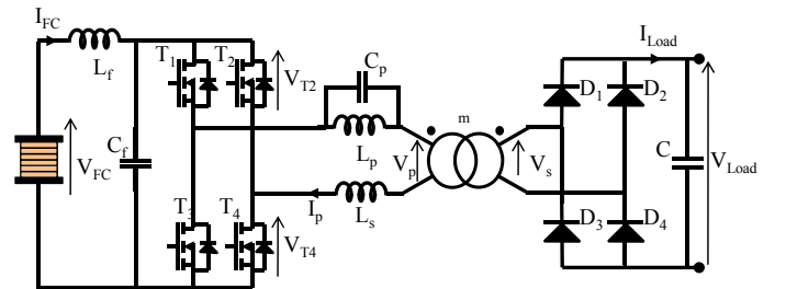
Fig. 15. Double resonant inverter topology.
