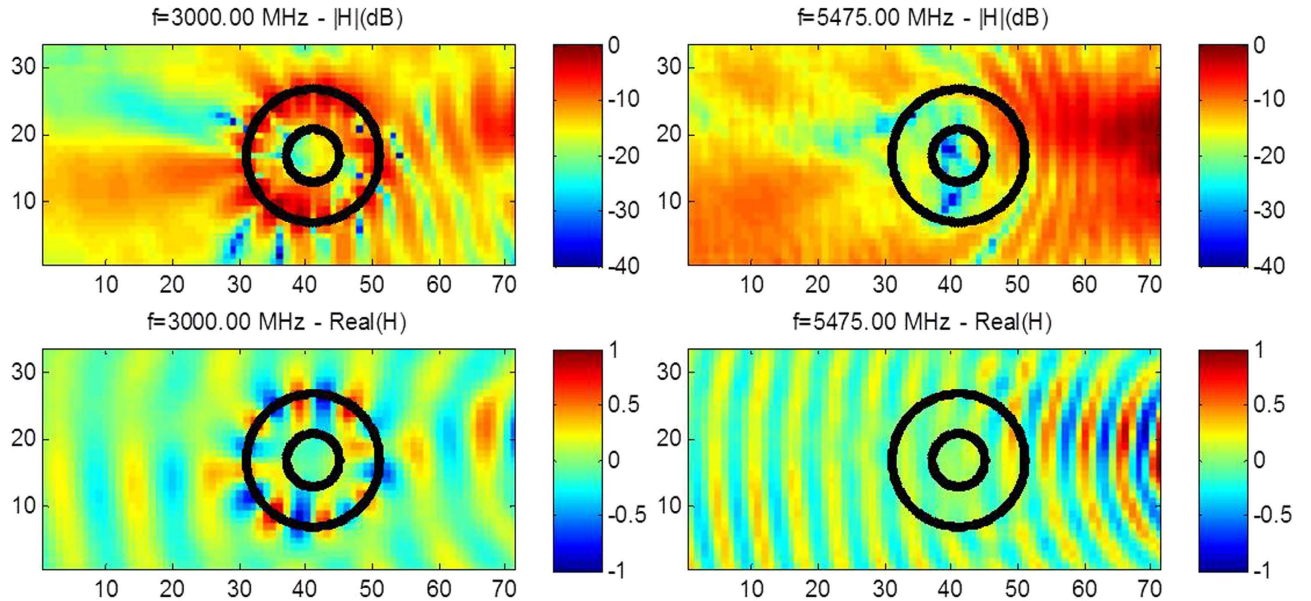
Figure 9. Experimental results for microwaves at two representative frequencies within the cloaking interval [2.6,6]GHz. The normalized modulus (upper panel) and the normalized real part (middle panel) of the magnetic field is measured for the source at 3 and 5.475 GHz. One notes that the magnetic field intensity is reduced by 17 dB and 30 dB at the center of the cloak with a reduction varying in the range [12.5,24] dB and [11,38] dB inside the inner disc, respectively at 3.5 and 5.475 GHz. The field is enhanced inside the corona at 3 GHz and both wavefront and field amplitude is better reconstructed behind the cloak at 5.475 GHz. Notably the measured intensity is -14 dB and -12 dB at the left side, respectively at 3 and 5.475 GHz and -1 dB at the right side, of the intensity panels. Protection is clearly more pronounced at 5.475 GHz than 3 GHz.
