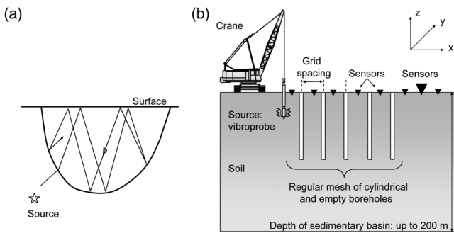
FIG. 1. Schematics of (a) a seismic wave in an alluvium basin and (b) the seismic testing device cross section in the x - z plane (see Fig. 3 for a photograph of the experiment).
