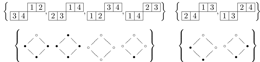
Fig. 1: The two orbits of \mathcal{L}([2] \oplus [2]) under \text{Pro} and of J([2] \times [2]) under \text{Row} .
