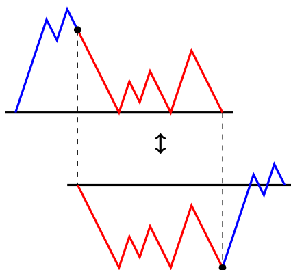
Fig. 1: Bijection between a pointed excursion (on top) and a pointed bridge.
