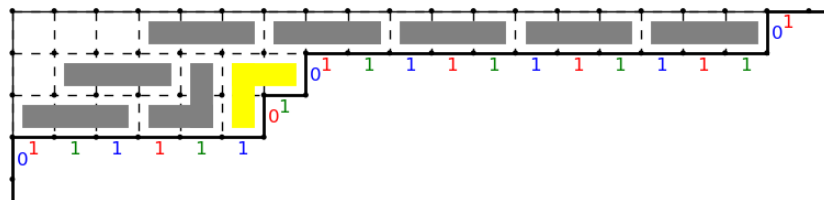
Fig. 2: The Young diagram of the partition \lambda = (18, 7, 6) together with its 01-sequence \dots 01111111010111111111101 \dots (the \mid indicates the unique location where the number of 1s to the left equals the number of 0s to the right, which is between index -1 and 0 in the 01-sequence; visually this corresponds to the main diagonal in the Young diagram). Notice the mnemonic “RGB” for the colourings, starting after the \mid mark. The grey shapes indicate a sequence of 3-hooks that can be removed from \lambda , to finally obtain the 3-core (3, 1) of \lambda . One could start with the yellow shape for instance, and then make various choices for the order of the removals. The process always ends with the same 3-core, (3, 1) (see Figure 1). Quotients will be \dots 0111011111 \dots (partition (2)), \dots 01111111 \dots (empty partition) and \dots 0111011101 \dots (partition (5, 2)). Remark that the yellow shape connects two labels in the 01-sequence that are blue. It thereby corresponds to a specific box of the quotient partition (5, 2) (see Figure 1 and compare with Equation (9)).
