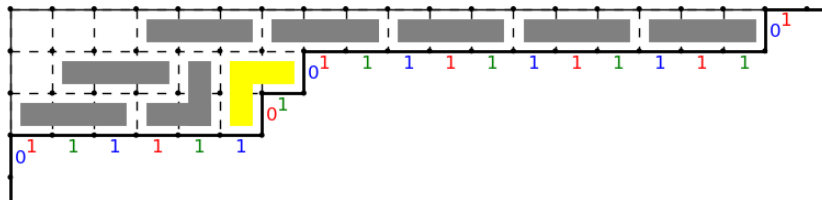
Fig. 2: The Young diagram of the partition \lambda = (18, 7, 6) together with its 01-sequence \dots 0111|111010111111111101 \dots (the | indicates the unique location where the number of 1s to the left equals the number of 0s to the right, which is between index -1 and 0 in the 01-sequence; visually this corresponds to the main diagonal in the Young diagram). Notice the mnemonic “RGB” for the colourings, starting after the | mark. The grey shapes indicate a sequence of 3-hooks that can be removed from \lambda , to finally obtain the 3-core (3, 1) of \lambda . One could start with the yellow shape for instance, and then make various choices for the order of the removals. The process always ends with the same 3-core, (3, 1) (see Figure 1). Quotients will be \dots 01|1011111 \dots (partition (2)), \dots 0|1111111 \dots (empty partition) and \dots 011|011101 \dots (partition (5, 2)). Remark that the yellow shape connects two labels in the 01-sequence that are blue. It thereby corresponds to a specific box of the quotient partition (5, 2) (see Figure 1 and compare with Equation (9)).
