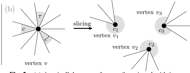
Fig. 2: (a) A unicellular map of genus 2 equipped with its corner labelling. Labels corresponding to trisections are boxed. (b) Given a trisection \tau , two other corners of interest c and c' are canonically defined (see text). “Slicing the trisection” then gives rise to three new vertices v_1, v_2, v_3 , with distinguished corners c_1, c_2, c_3 . (c) The recursive procedure of [3]: if c_3 is the minimum corner of v_3 , then stop; else, as shown in [3], c_3 is a trisection of the new map M' : in this case, iterate the slicing operation on (M', c_3) .
