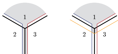
Fig. 5: Approximating neighbourhoods corresponding to a = 1 and b = 23 (on the left), respectively a = 1 and b = 123 (on the right).
