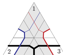
Fig. 6: An approximating neighbourhood for a = 1, b = 23 as an intersection of affine pseudohalfspaces in a blow-up of the black tropical pseudohyperplane.
