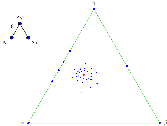
Figure 4: Picture of \widehat{Q} and the first normalized roots (with depth \leq 12 ) for the Coxeter root system of type \widetilde{G}_2 (affine).
